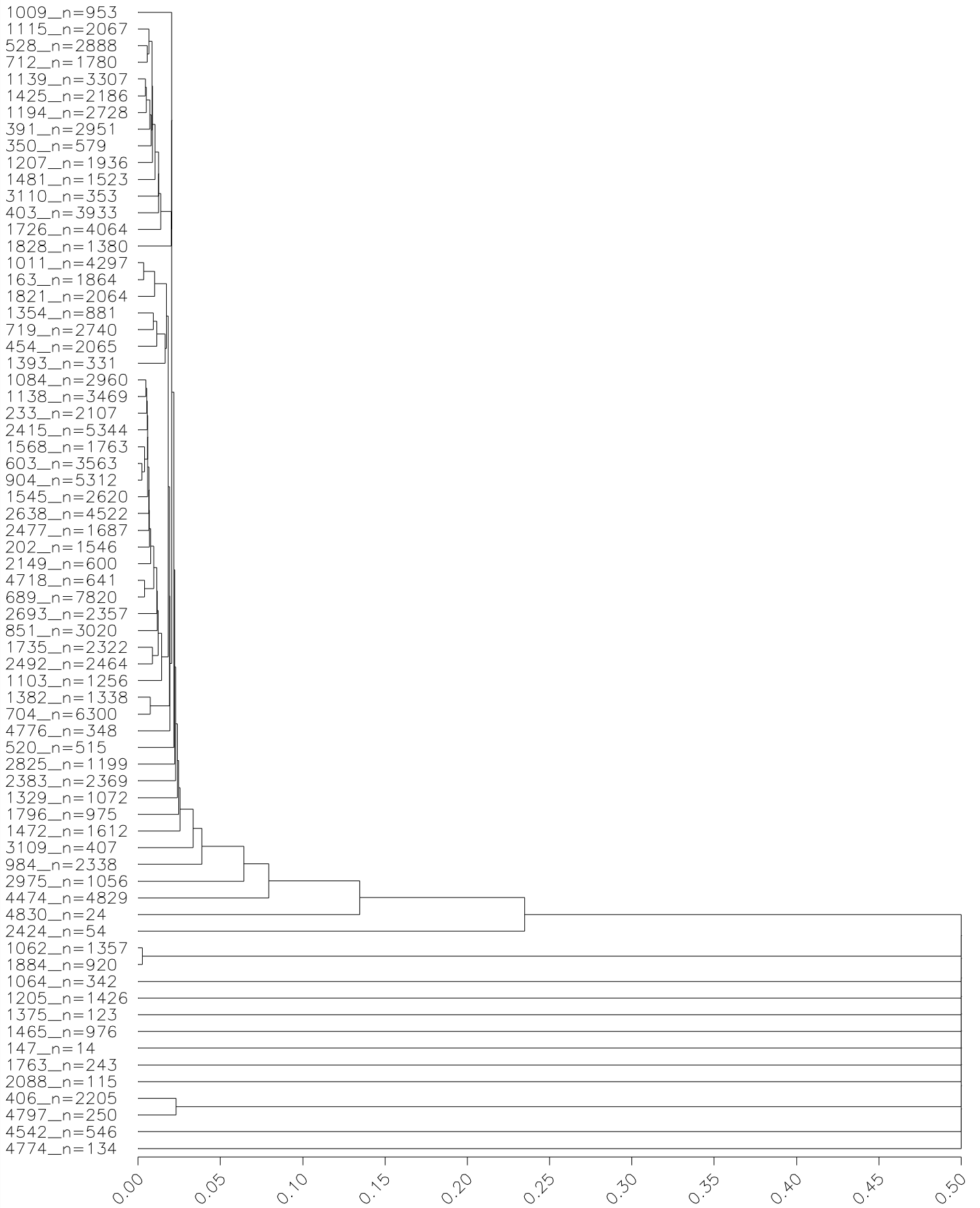
Connectedness distances for WOOL from 2002 to 2006 – GEJob 13929
