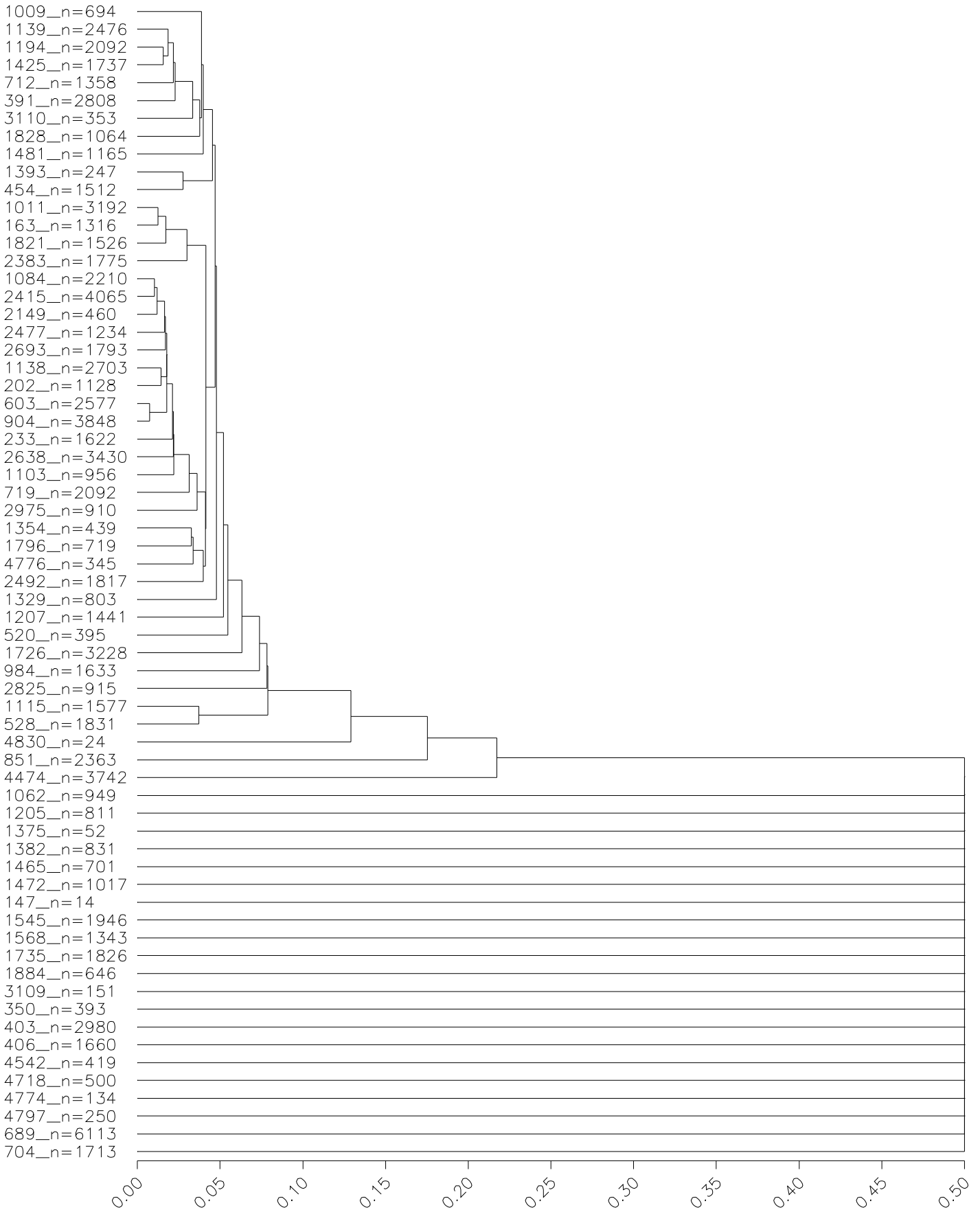
Connectedness distances for MEAT from 2003 to 2006 – GEJob 13929
